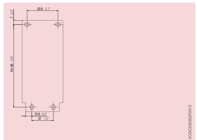
DB96 - drilling plan
