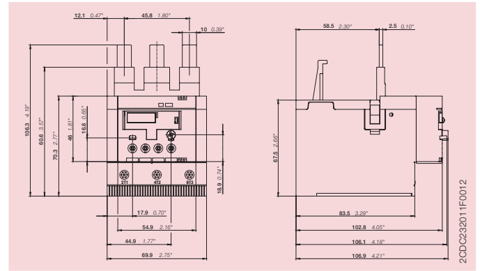
TF96 dimension drawing
