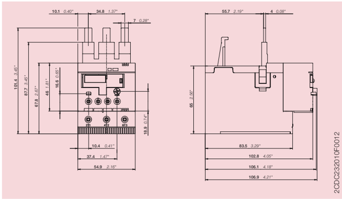
TF65 dimension drawing
