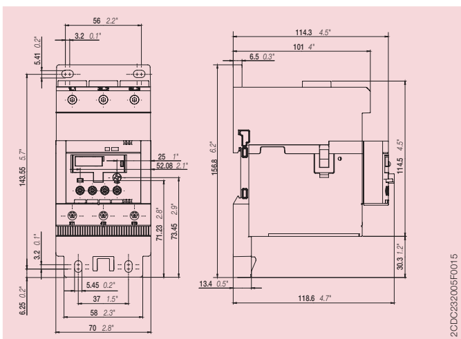
DB96 - dimension drawing - Single mounting kit + Electronic overload relay TF96
