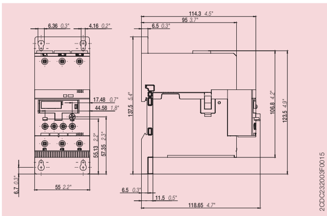
DB65- dimension drawing - Single mounting kit + overload relay TF65
