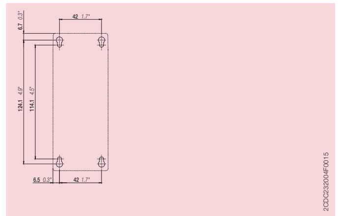
DB65 - drilling plan
